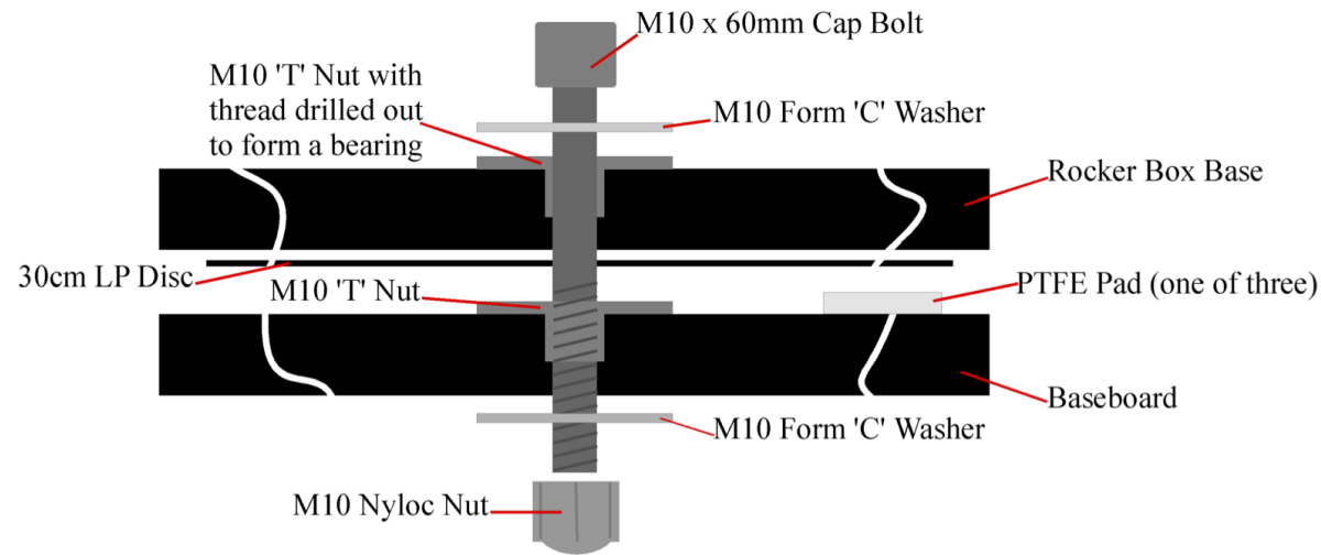
AZIMUTH BEARING ASSEMBLY
